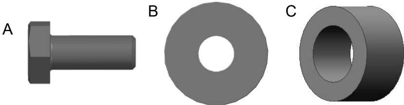
A. Bolt M10x1.5x30.....Qty 4 B. Washer M10.....Qty 4 C. Spacer 6 mm.....Qty 2
